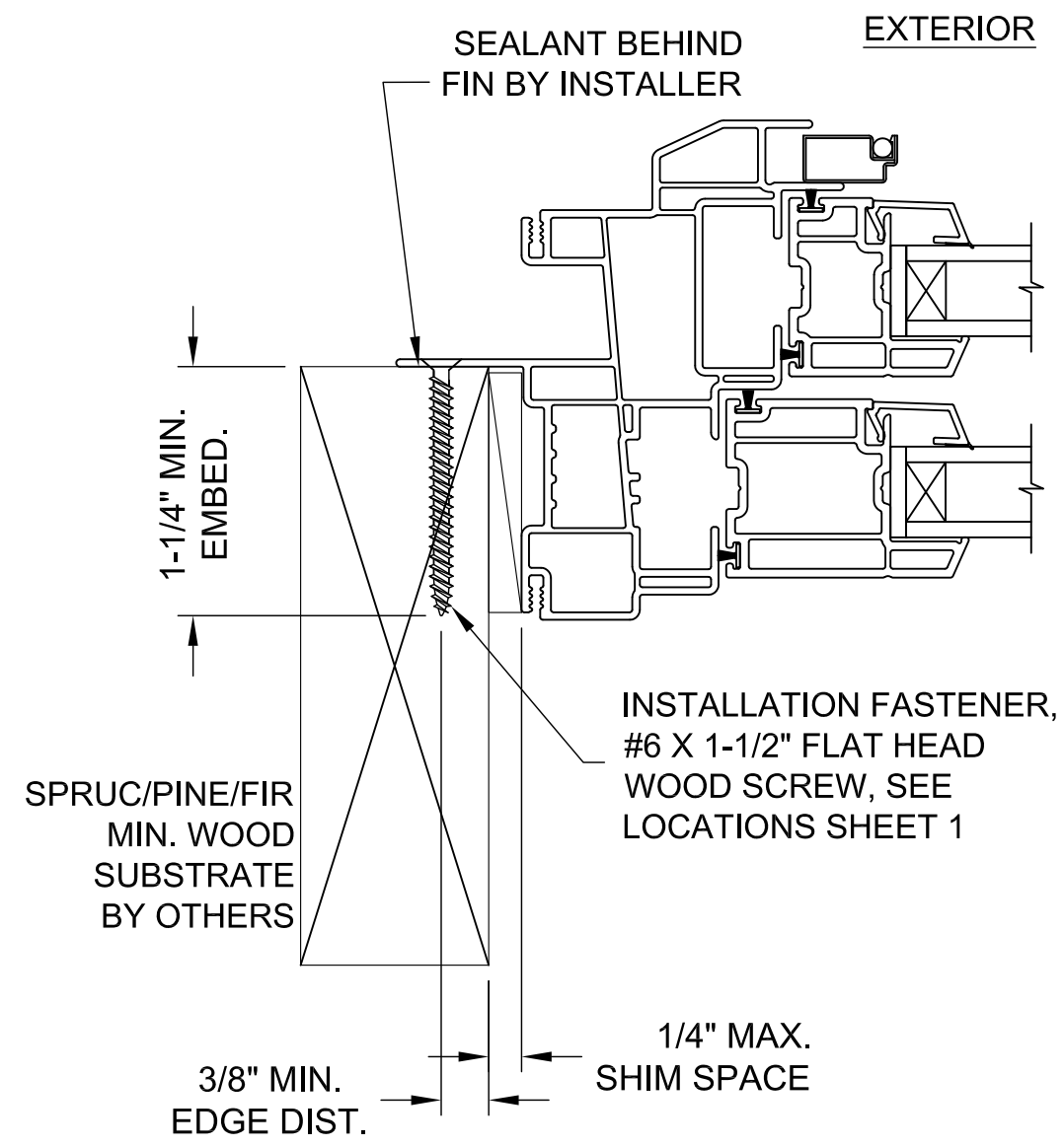
TYPICAL JAMB HORIZONTAL SECTION
