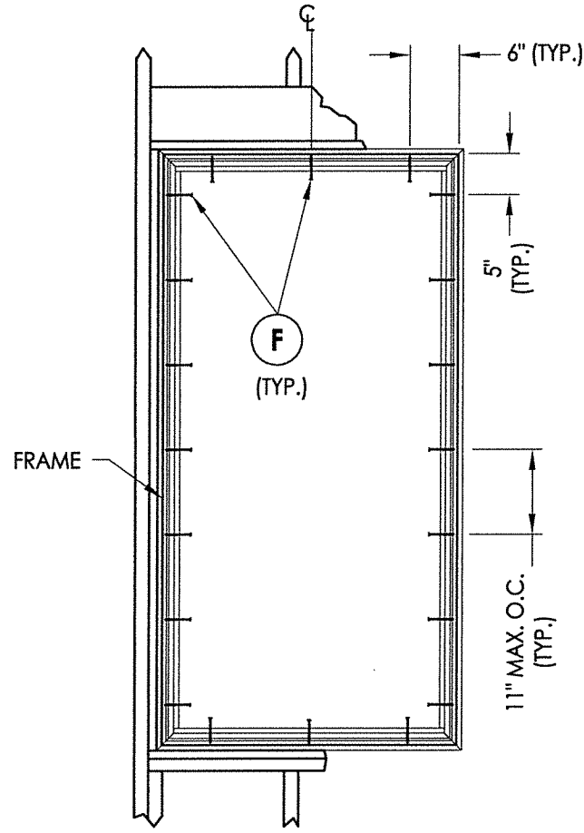
FRAME ANCHORING 36" x 72" MAX. FRAME SIZE
