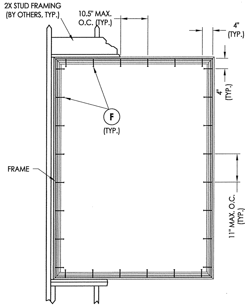
FRAME ANCHORING 60" x 84" MAX. FRAME SIZE
