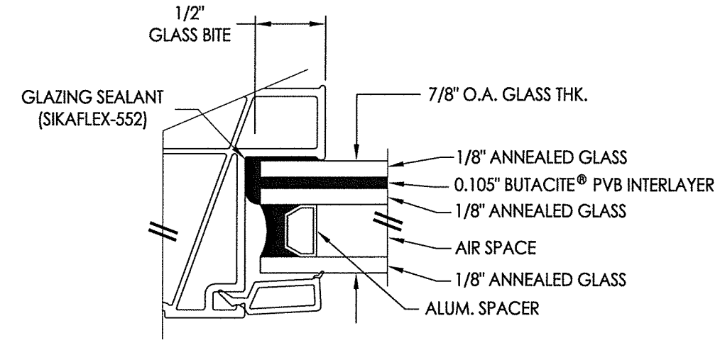
G3 GLAZING DETAIL
