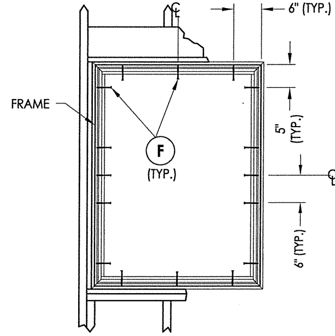
FRAME ANCHORING 36" x 48" MAX. FRAME SIZE
