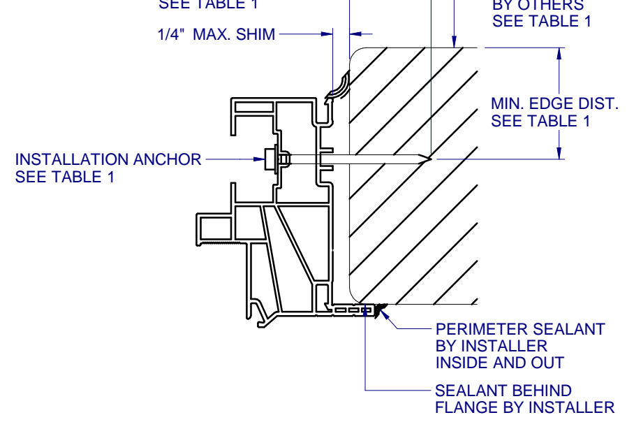
B HORIZONTAL SECTION 7 TYPICAL JAMB ANCHORAGE
