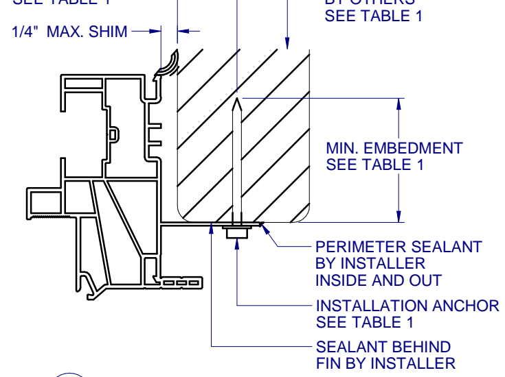
C HORIZONTAL SECTION 7 TYPICAL FIN ANCHORAGE HEAD AND SILL SIMILAR FOR FIN INSTALLATION
