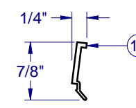
PVC GLAZING BEAD-6064
