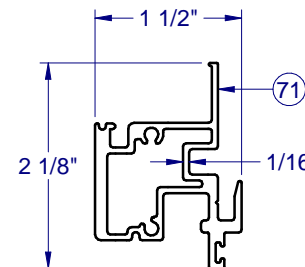
FIXED RAIL - 1836
