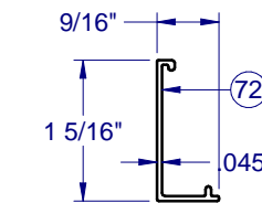
PVC FIXED RAIL COVER - 6063
