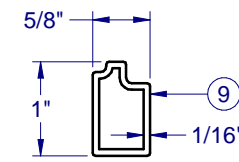
REINF. TOP RAIL-1497
