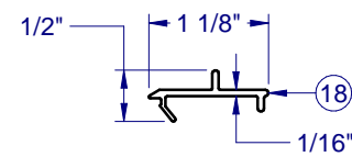
PVC SCREEN CATCH - 6013
