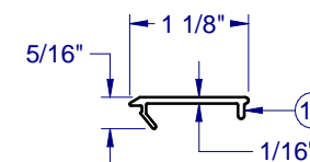
PVC SCREEN SUPPORT - 6014
