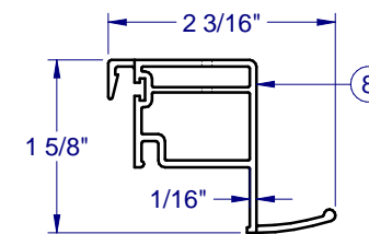
PVC SASH TOP RAIL-6027
