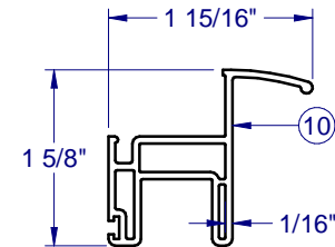
PVC SASH BTM. RAIL-6028
