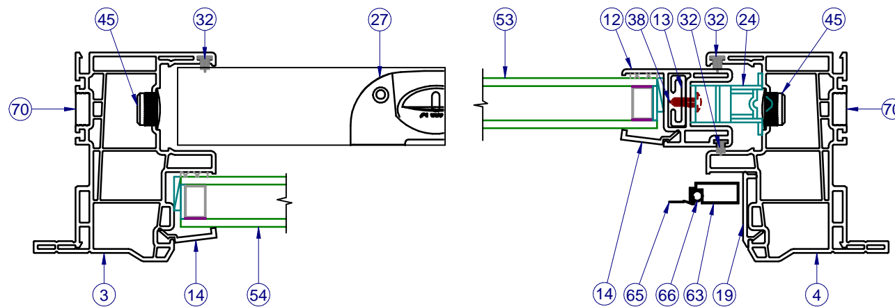
SECTION B-B
