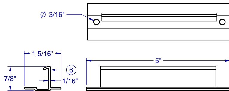
IMPACT HOOK S-1577
