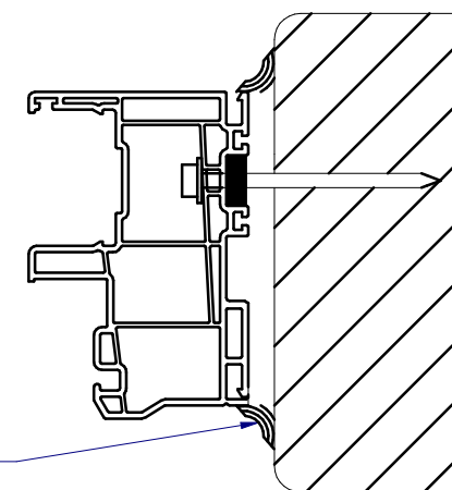
C 6 HORIZONTAL SECTION BOX FRAME INSTALLATION HEAD AND SILL SIMILAR FOR BOX INSTALLATION
