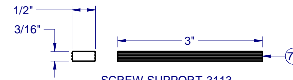
SCREW SUPPORT-3113
