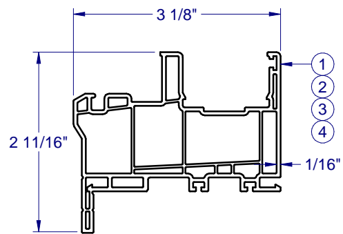
PVC FRAME FLANGE-6031
