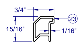
REINF. BTM RAIL-1699
