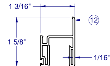
PVC SASH SIDE RAIL - 6004
