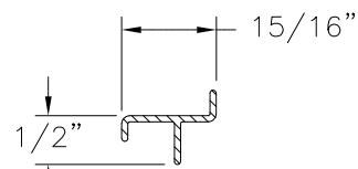
SASH REINFORCEMENT ALUMINUM 6063-T5 (10500006)
