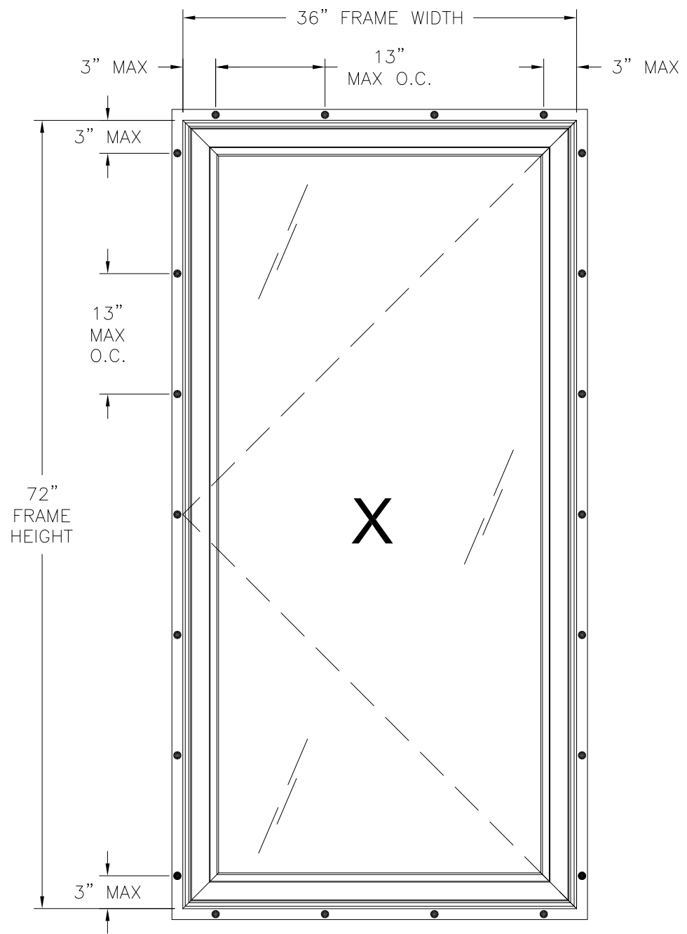
4325 CASEMENT WINDOW EXTERIOR VIEW FIN INSTALLATION
