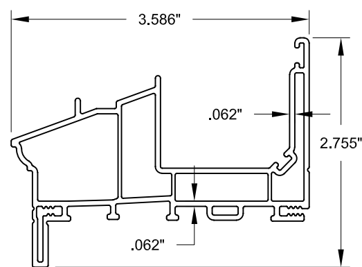
2 SILL, W/FLANGE
