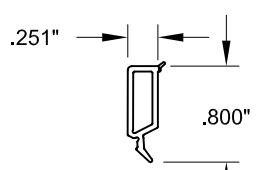
17 FIXED LITE GLAZING BEAD
