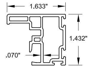
10 SASH STILE
