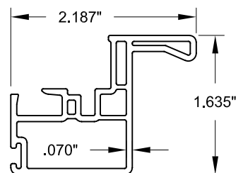
9 LIFT RAIL
