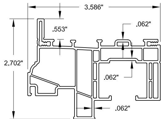
1 HEAD & JAMB, W/FLANGE
