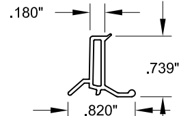
19 SASH GLAZING BEAD WITH DRIP EDGE (OPTIONAL)
