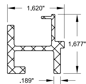
11 REINFORCEMENT (MEETING RAIL)
