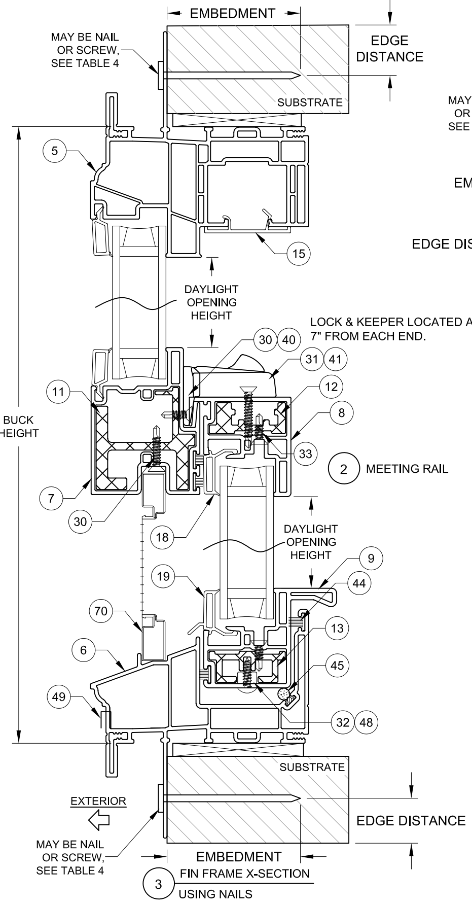
1 FIN FRAME X-SECTION USING NAILS
