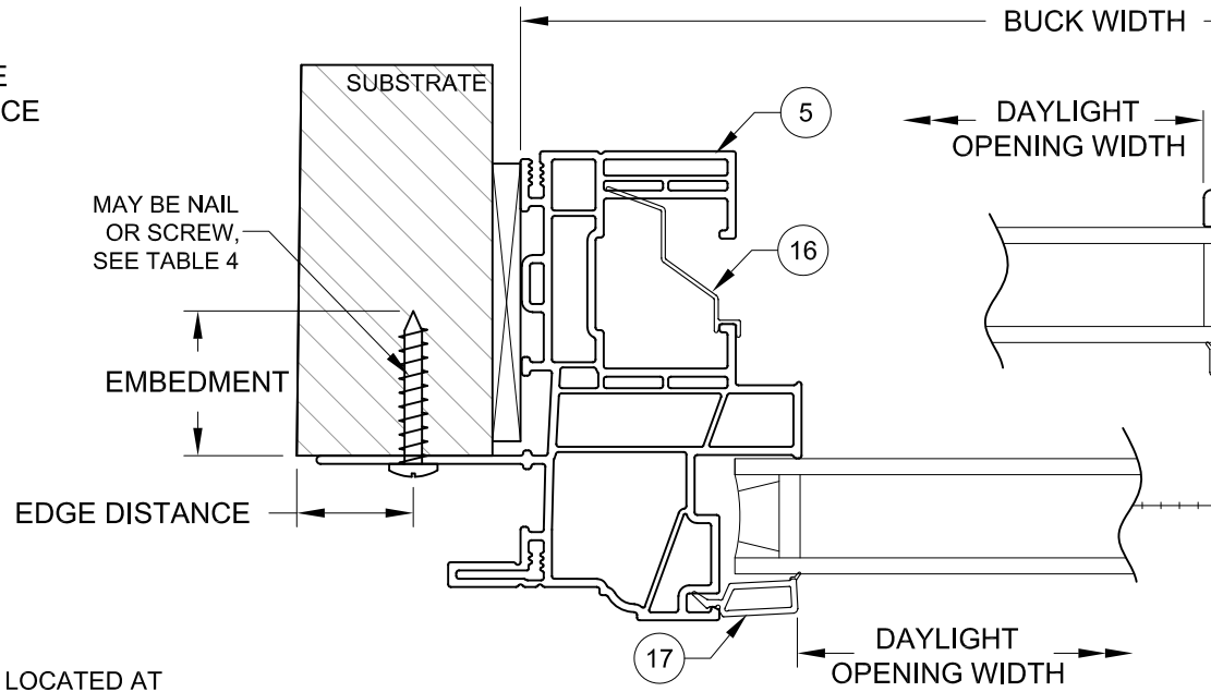
4 FIN FRAME X-SECTION USING SCREWS
