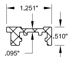
12 REINFORCEMENT (LOCK RAIL)
