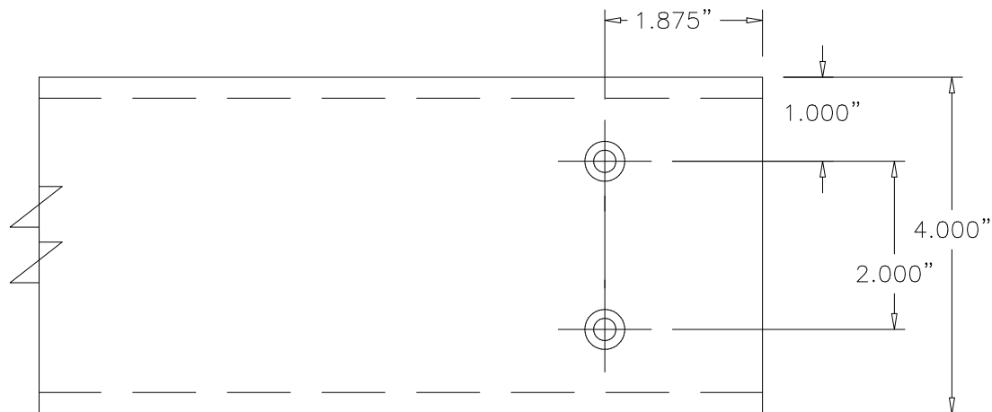
MULLION ALUMINUM 6063-T6 .25" THICK
