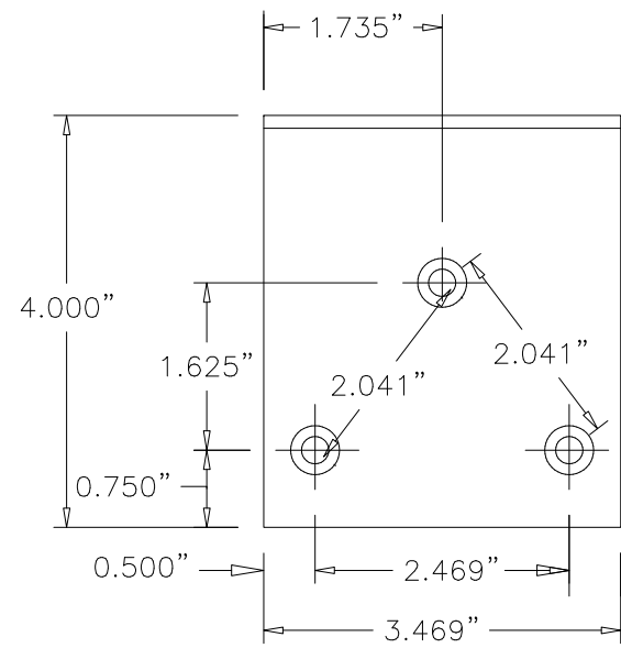
CLIP ALUMINUM 6105-T5 .125" THICK
