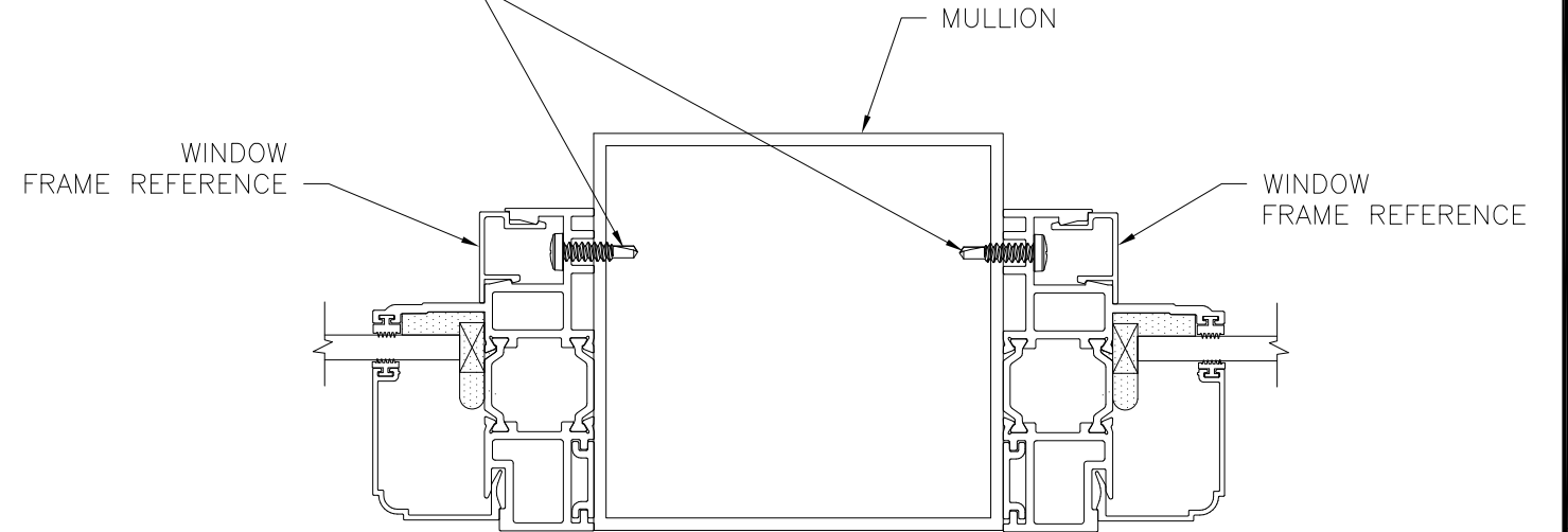
WINDOW/MULLION CONNECTION DETAIL
