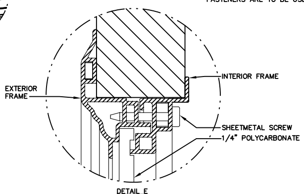
DETAIL E
