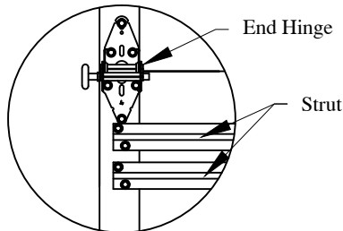
Additional Strut below hinge
