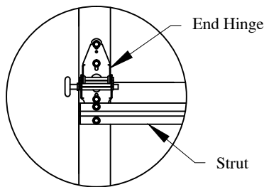
Strut on bottom half of hinge Detail C
