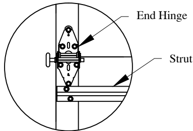
Strut below hinge Detail C
