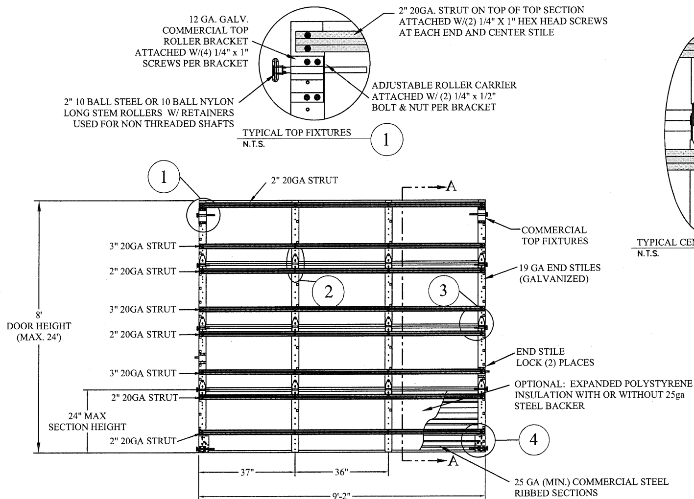
DOOR INTERIOR ELEVATION
