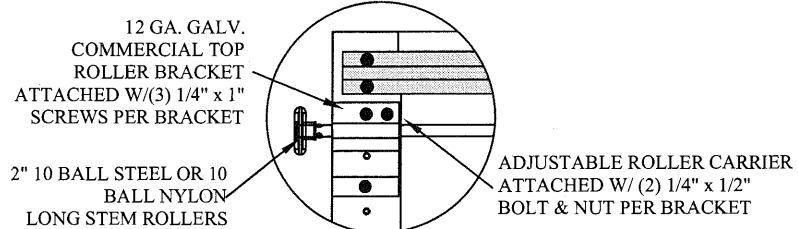
TYPICAL TOP FIXTURES N.T.S. 1
