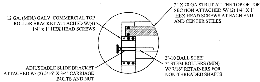
TYPICAL TOP FIXTURES N.T.S.
