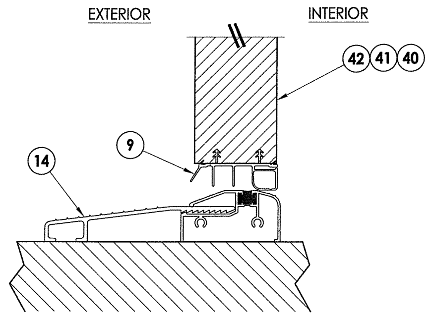
3 VERTICAL CROSS SECTION 4 Inswing configuration
