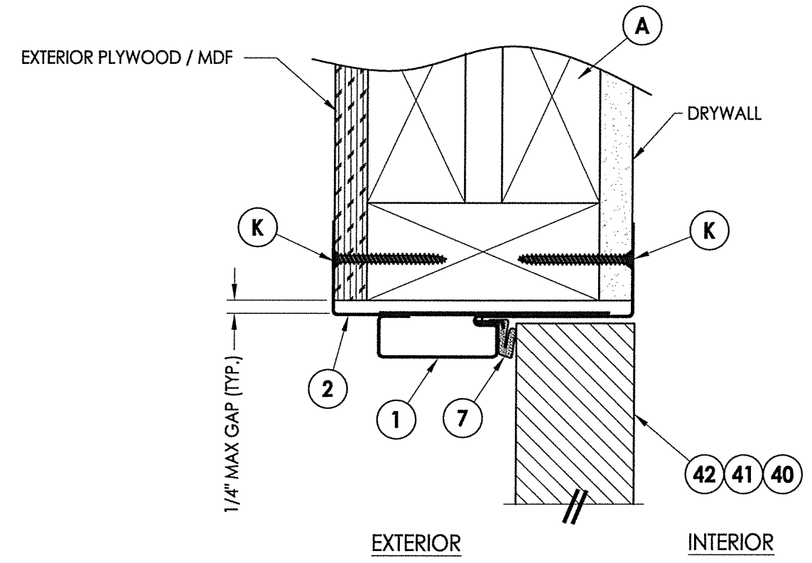
1 VERTICAL CROSS SECTION 4 Inswing shown (Outswing similar)
