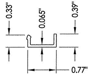
8 3/4" GLAZING BEAD
