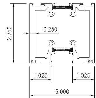
2 FRAME
