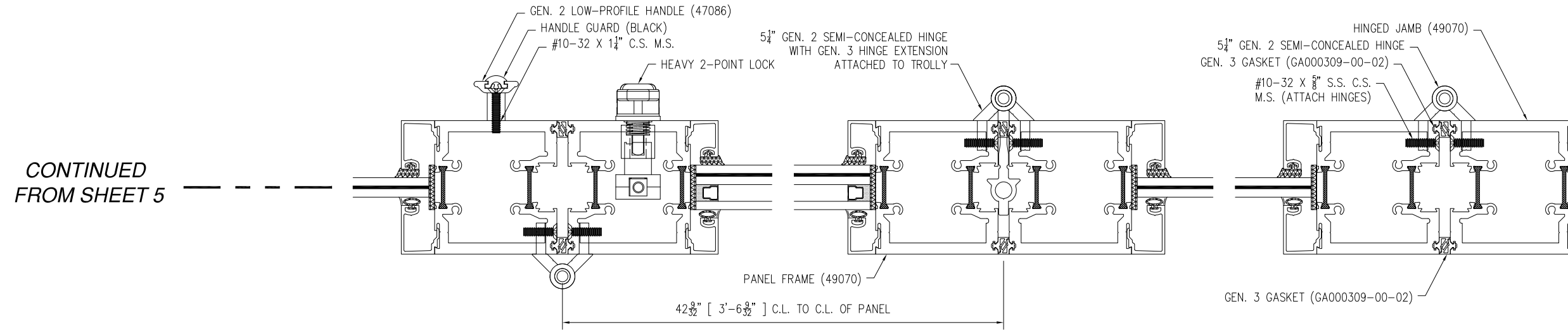
HORIZONTAL CROSS SECTION
