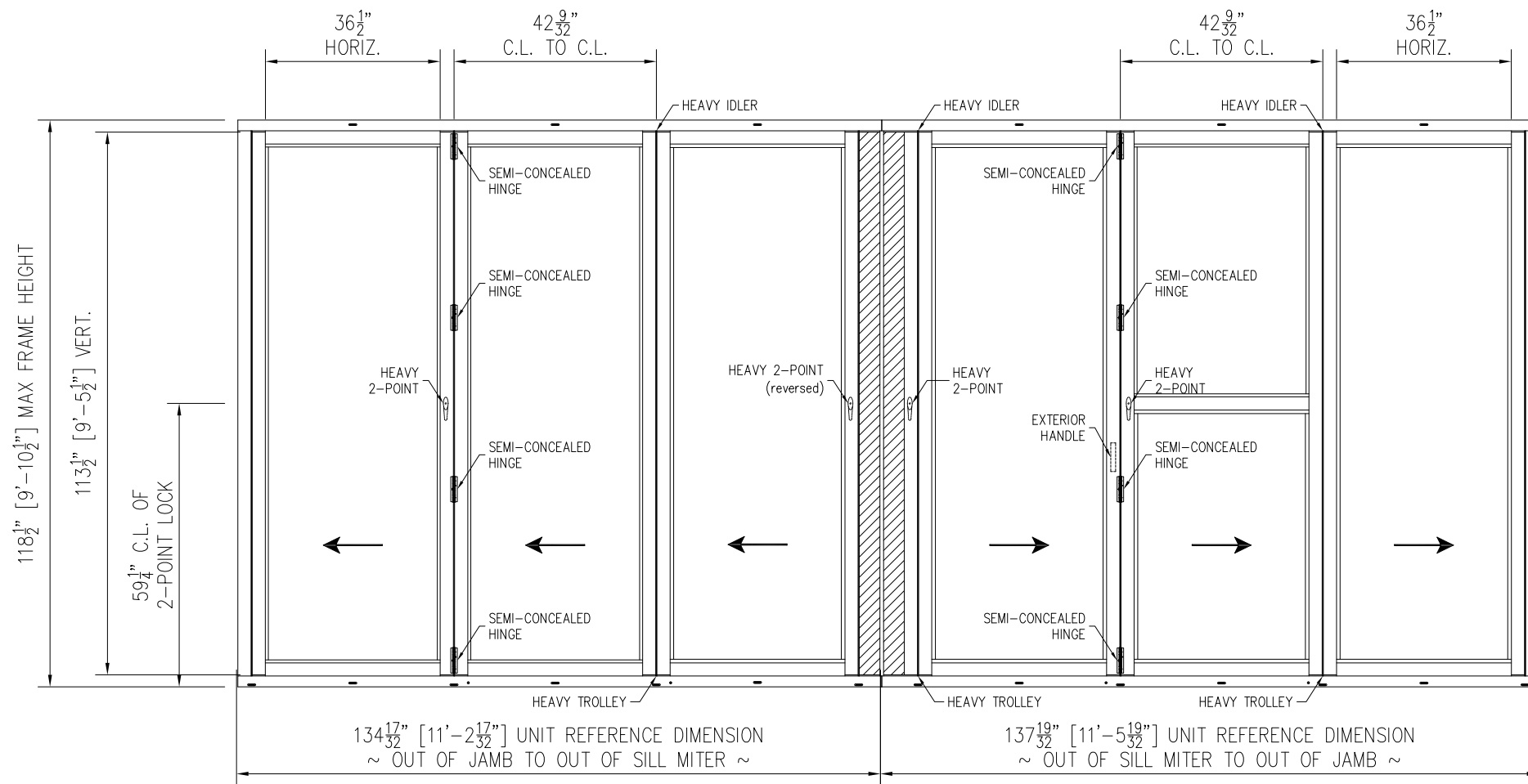
SI 33350 G3 IMPACT FGW 3.5X9.5 PANEL 90° CORNER NO-POST - FLUSH SILL EXTERIOR VIEW
