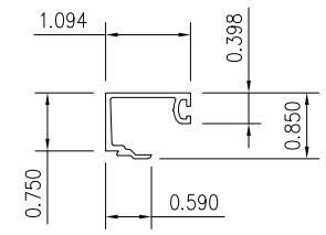
9 7/16" GLASS STOP
