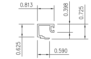
8 1/4" GLASS STOP
