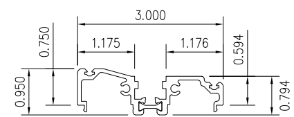
7 3rd GENERATION DOOR ADAPTOR
