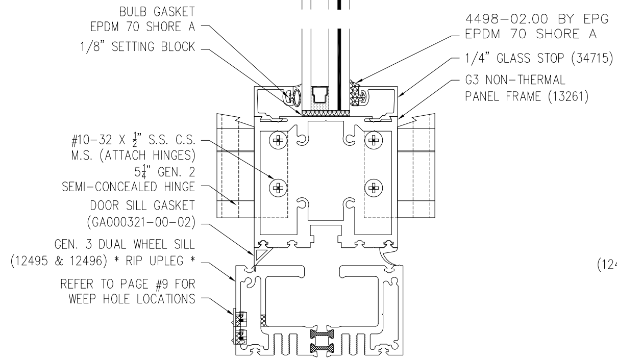
VERTICAL CROSS SECTION STANDARD
