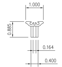
10 2nd GENERATION HANDLE
