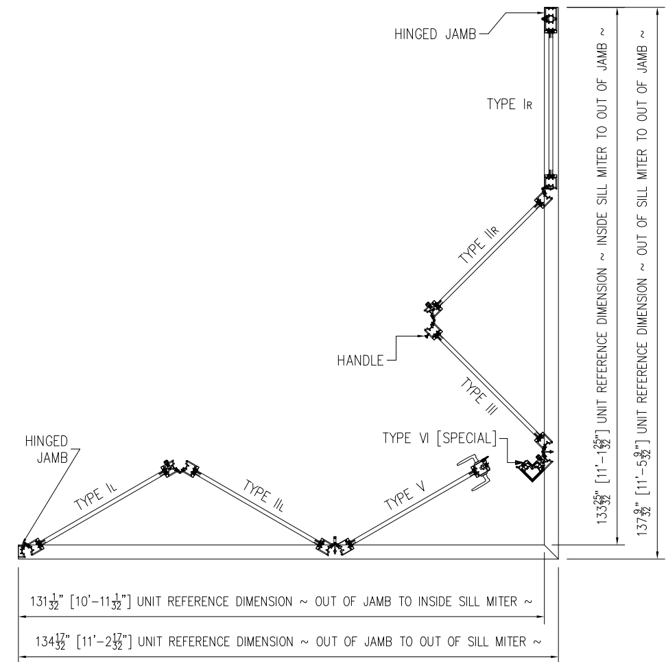
SI 33350 G3 IMPACT FGW 3.5X9.5 PANEL 90° CORNER NO-POST - FLUSH SILL PLAN VIEW
