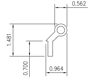
16 5 1/4" SEMI-CONCEALED HINGE
