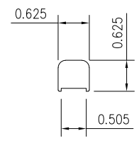
14 IDLER BODY
