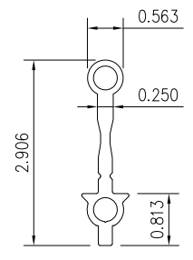
12 HINGE EXTENSION
