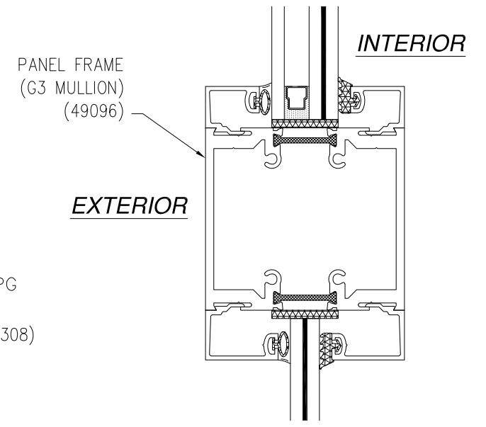
VERTICAL CROSS SECTION HORIZONTAL RAIL OPTIONAL
