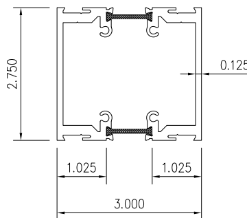
4 HORIZONTAL MULLION
