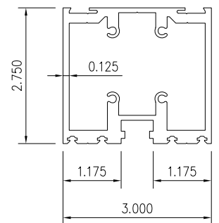
3 NON-THERMAL FRAME
