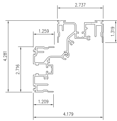
11 KNUCKLE JAMB
