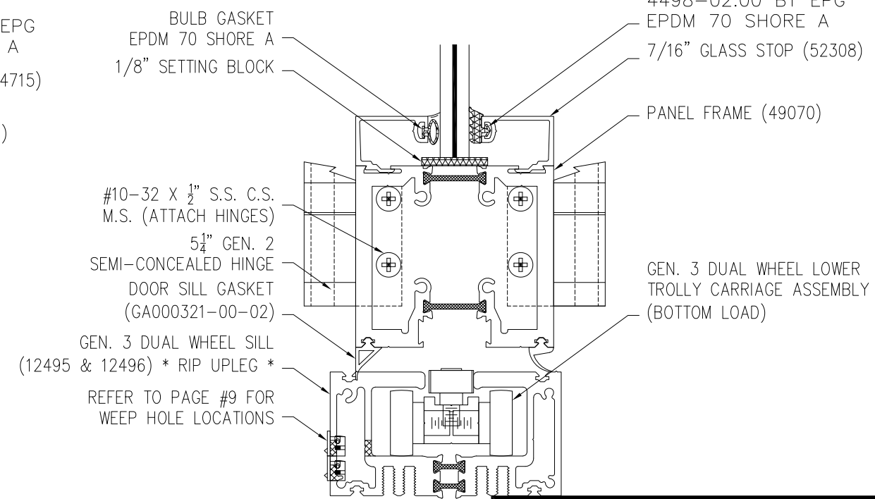
VERTICAL CROSS SECTION BOTTOM LOAD SILL
