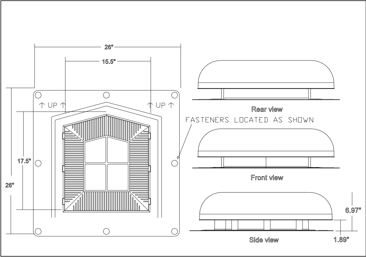
Figure 1. Fastener Locations.
