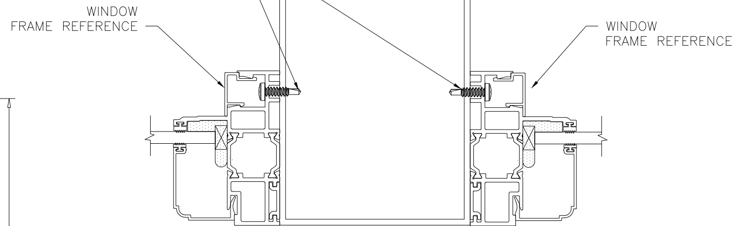
WINDOW/MULLION CONNECTION DETAIL
