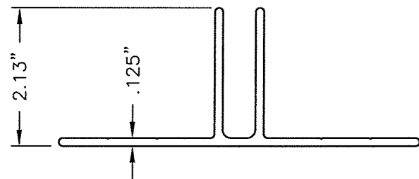
MULLION ANCHOR BRACKET MAT'L: 6063-T6
