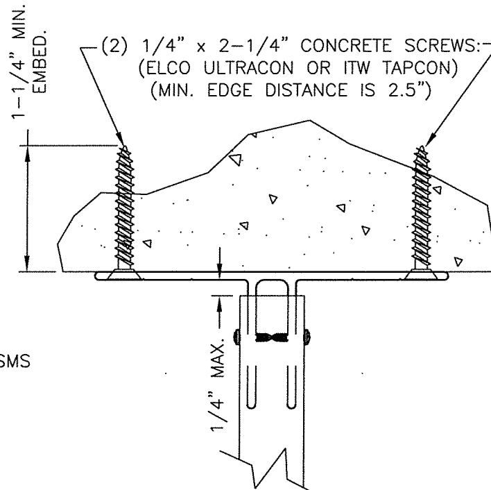
ANCHOR TO MASONRY USING 1/4" X 1-3/4" CONCRETE SCREWS
