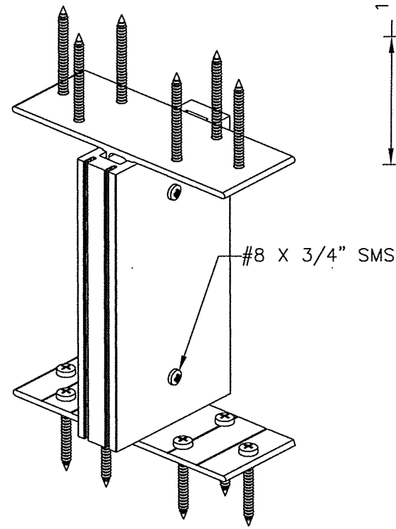
BASIC MULLION BRACKET ANCHORING FOR WOOD SCREW CONNECTIONS
