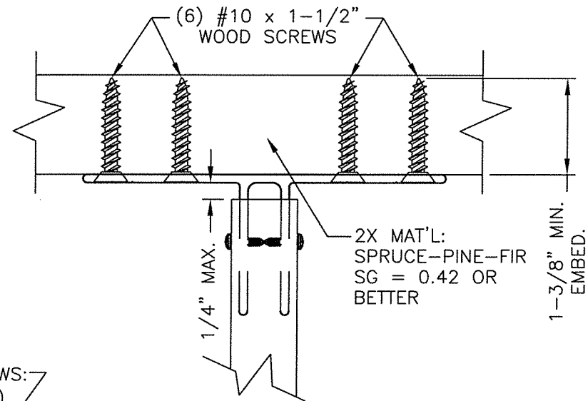
ANCHOR TO 2X STUD OR TO 2X BUCK USING #10 X 1-1/2" WOOD SCREWS
