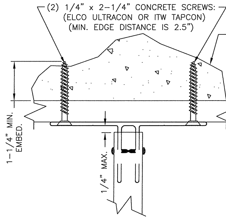
ANCHOR THROUGH 1X BUCK USING 1/4" X 2-1/4" CONCRETE SCREWS
