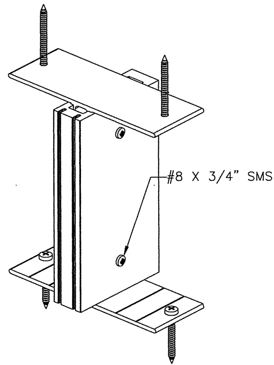
BASIC MULLION BRACKET ANCHORING FOR CONCRETE SCREW CONNECTIONS
