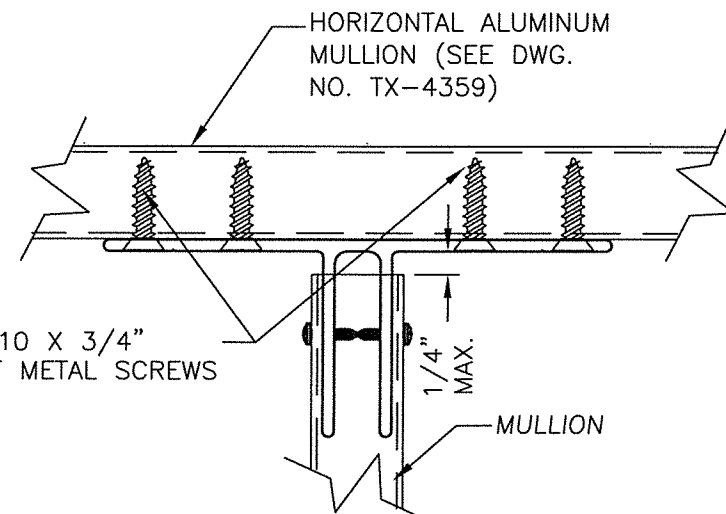
ANCHOR MULLION TO MULLION
