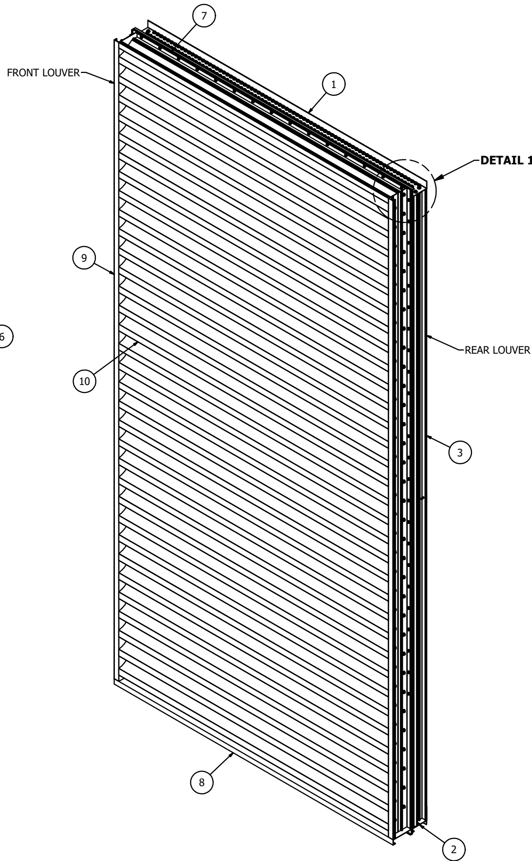
DETAIL 1 LOUVER ASSEMBLY
