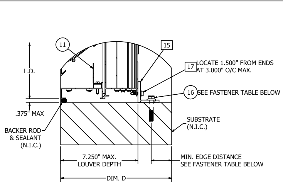
DETAIL 3 ANGLE INSTALL AT SILL
