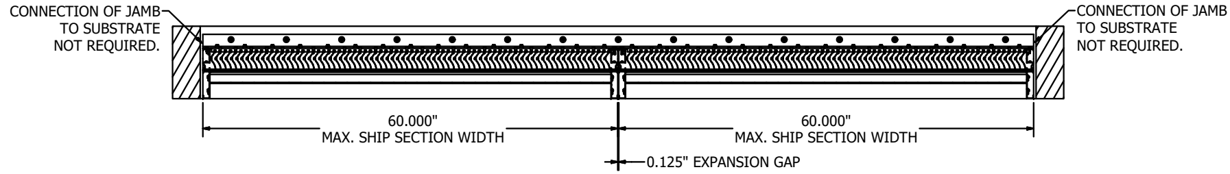
SECTION B-B
