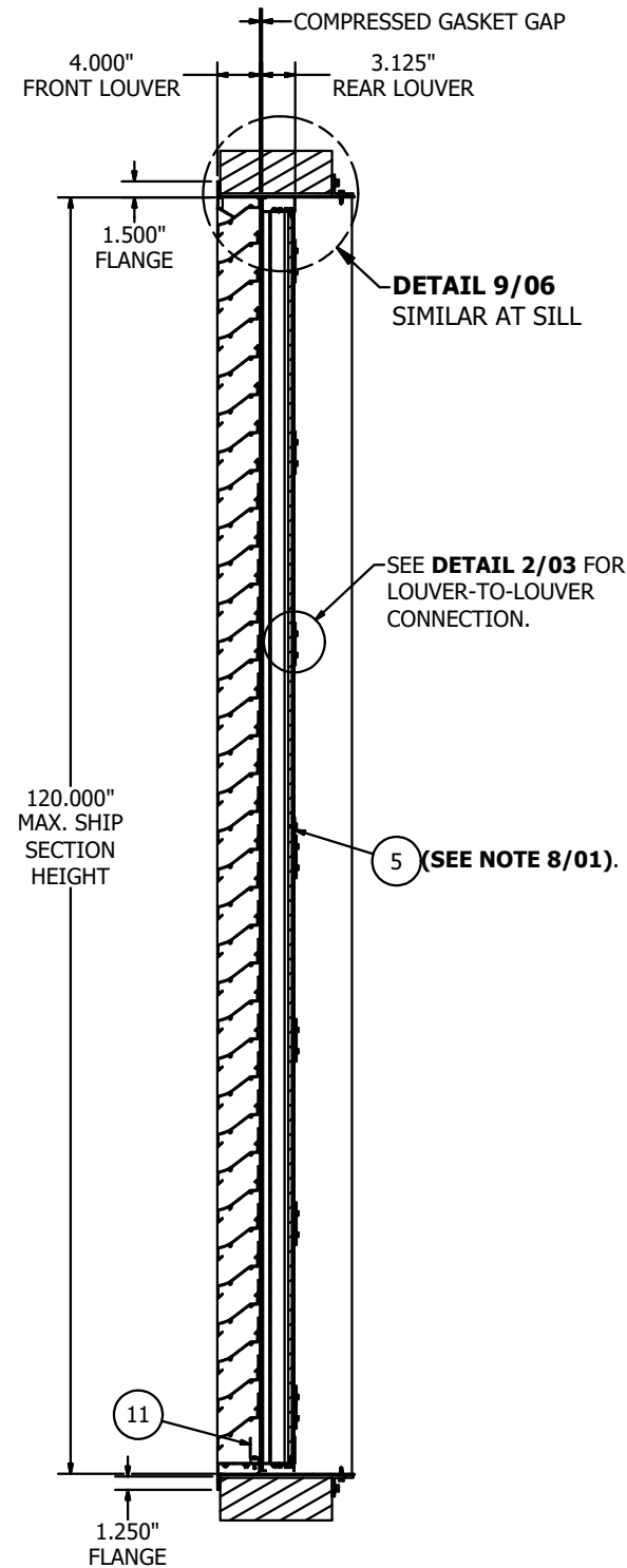
SECTION C-C
