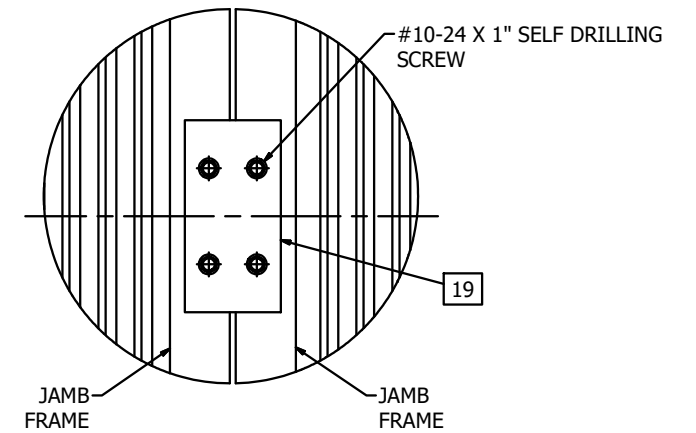
DETAIL 2 LOUVER-TO-LOUVER SPLICE
