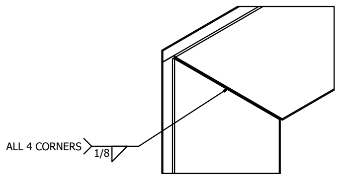
UNIVERSAL SLEEVE CORNER WELDS
