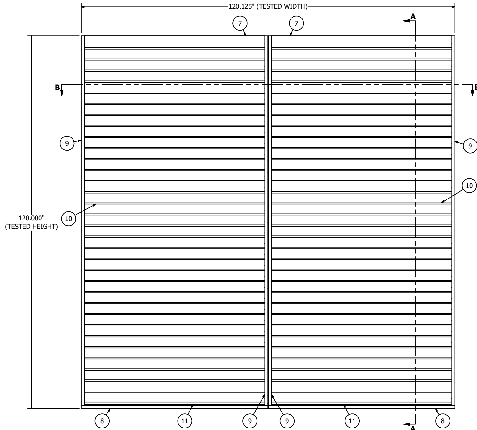
MULTI-SECTION ASSEMBLY - CHANNEL FRAME (FRONT) LOUVER
