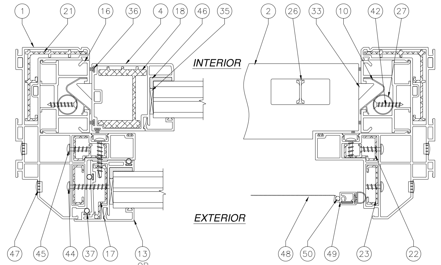
B 3 HORIZONTAL CROSS SECTION TRIPLE GLAZED SHOWN, DOUBLE GLAZED SIMILAR
