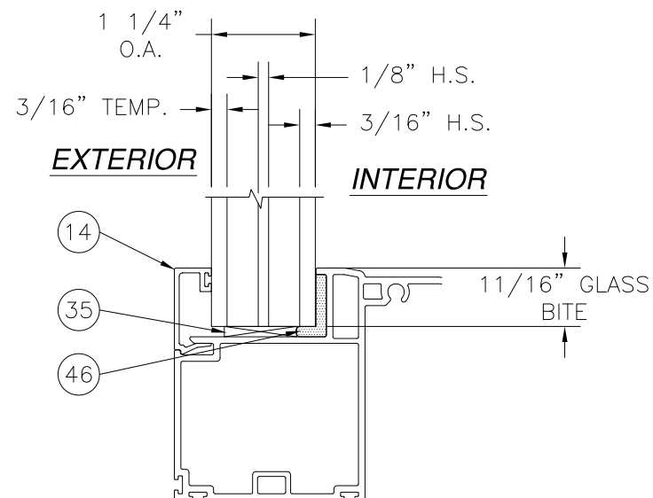
GLAZING OPTION B
