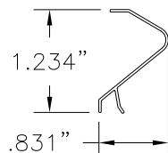
10 BALANCE COVER EXTRUDED RIGID PVC .030" THICK
