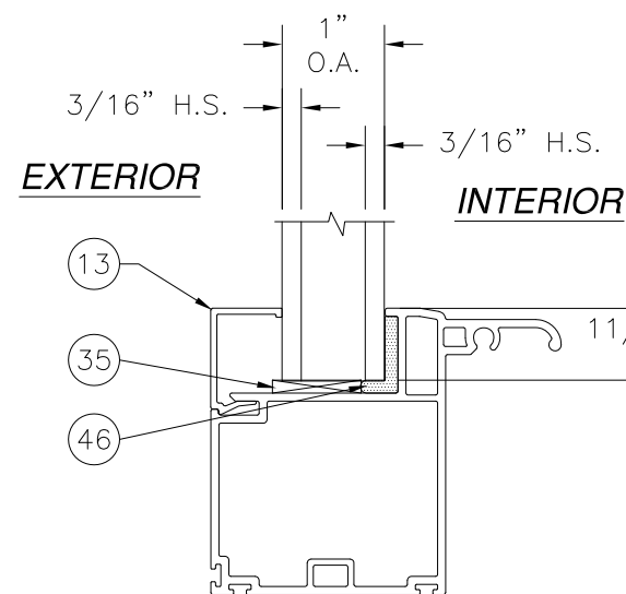
GLAZING OPTION A
