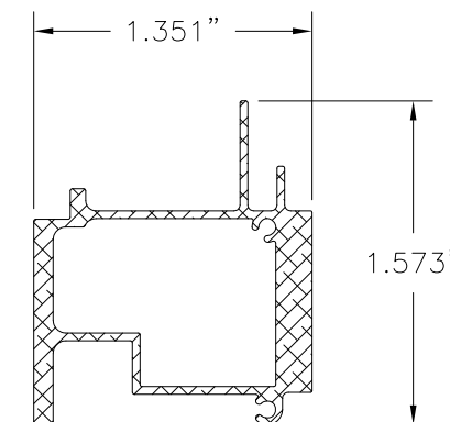
24 FIXED SASH REINFORCEMENT ALUMINUM 6063-T6 .075" THICK
