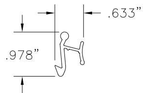
26 SNAP LATCH HANDLE EXTRUDED RIGID PVC .050" THICK
