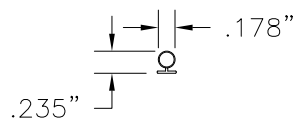
37 FIXED SASH BULB SEAL VINYL
