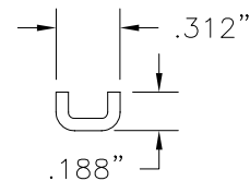
29 TILT BALANCE PIVOT BAR .060" THICK
