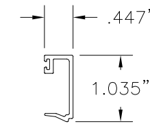
14 1 1/4" GLASS STOP EXTRUDED RIGID PVC .059" THICK
