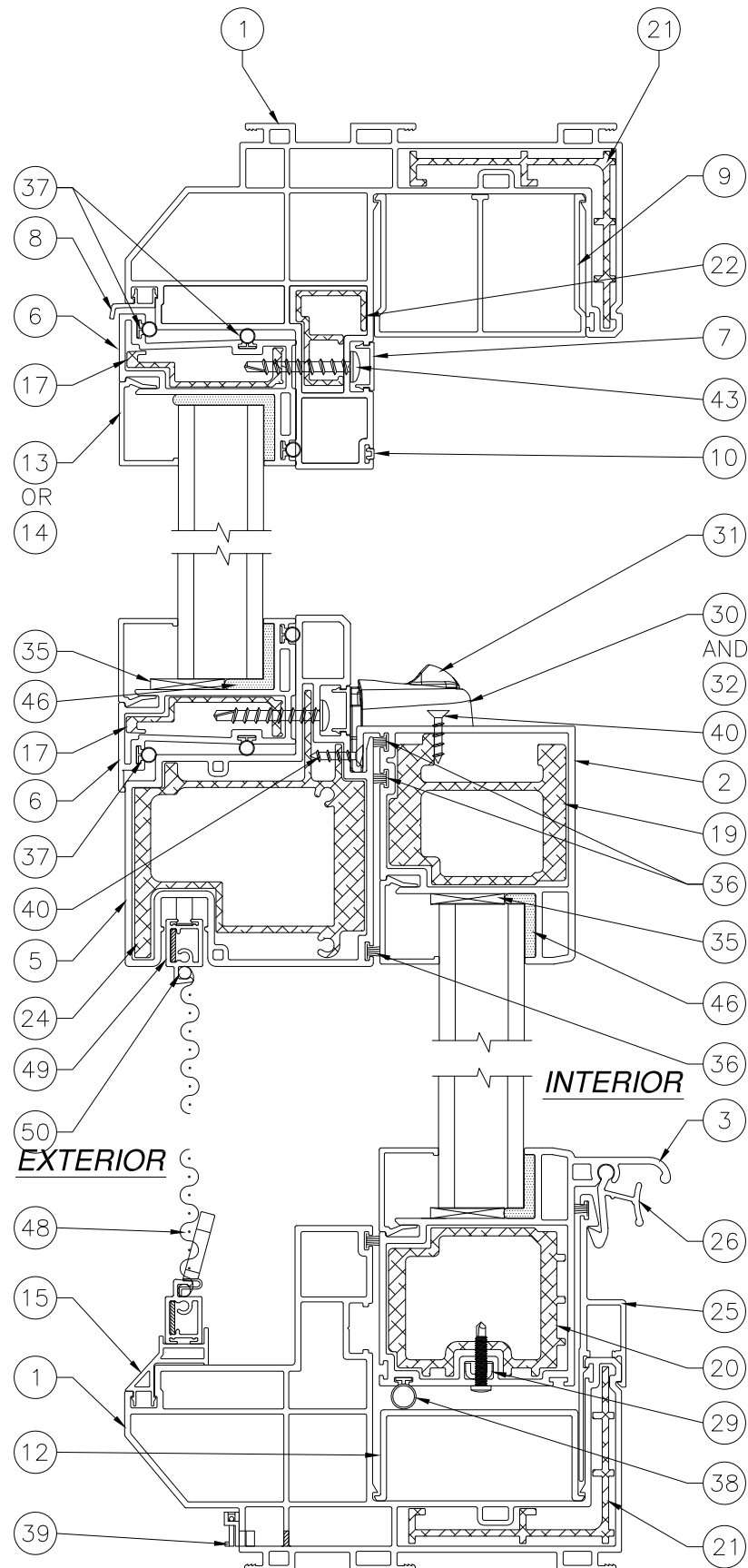
A 3 VERTICAL CROSS SECTION DOUBLE GLAZED SHOWN, TRIPLE GLAZED SIMILAR
