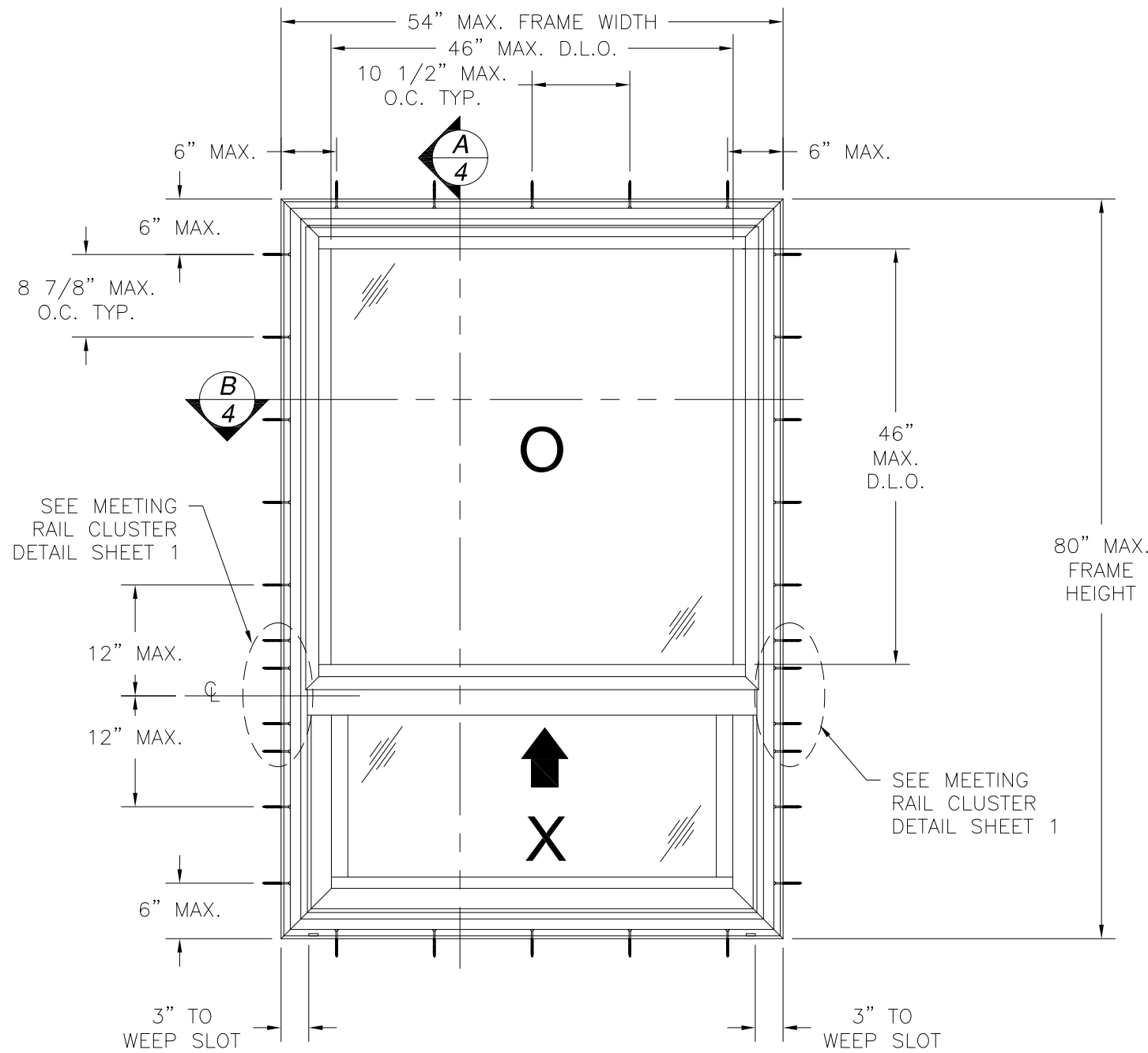
SERIES V-200 PVC SINGLE HUNG ORIEL WINDOW EXTERIOR VIEW
