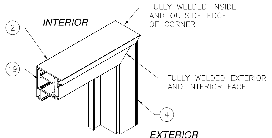
SASH CORNER CONSTRUCTION DETAIL
