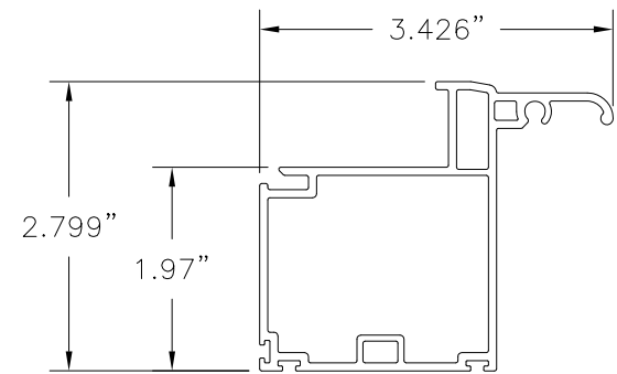
3 SASH BOTTOM RAIL EXTRUDED RIGID PVC .079" THICK
