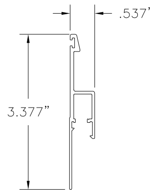
25 SILL WATERDAM EXTENDER EXTRUDED RIGID PVC .060" THICK
