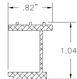
18 SASH STILE REINFORCEMENT ALUMINUM 6063-T6 .095" THICK
