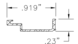
17 FIXED SASH REINFORCEMENT ALUMINUM 6063-T6 .060" THICK
