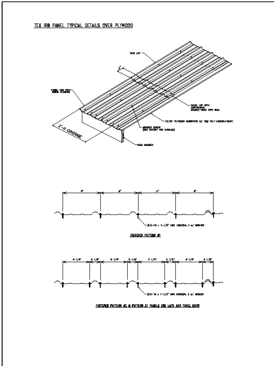
Figure 1. Tex Rib Panel Secured to Minimum 15/32" Plywood
